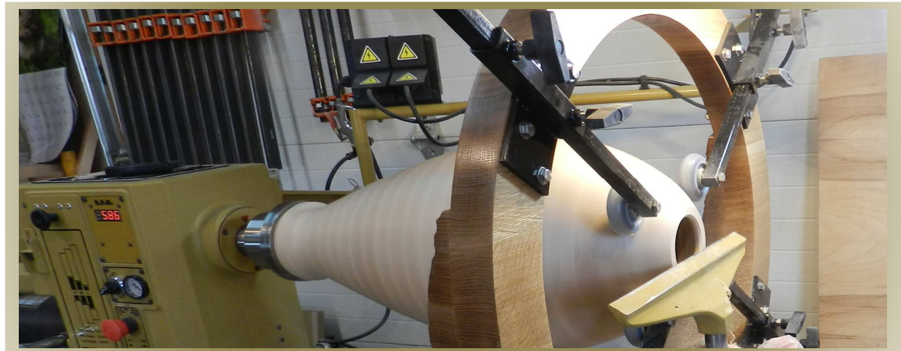
MLW Steady Rest in use
